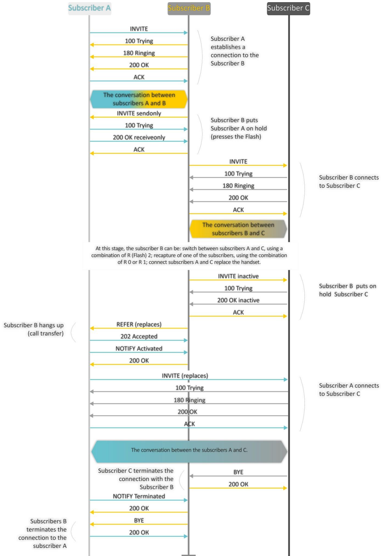
Figure below shows 'Attended calltransfer' service operation algorithm.
