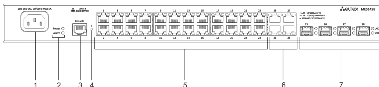
Figure 1 — MES1428 AC front panel
