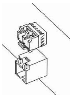
Figure 61 — Installed SFP transceivers
