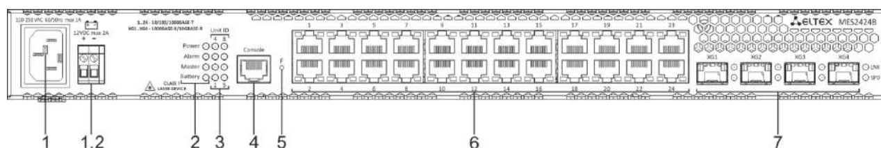
Figure 20 — MES2424B front panel
