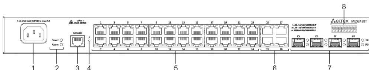
Figure 17 — MES2428T front panel
