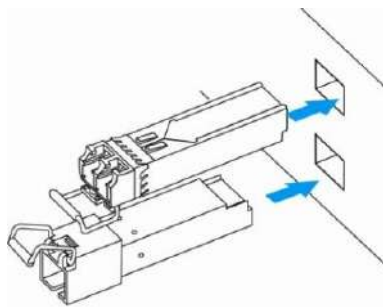
Figure 60 — SFP transceiver installation
