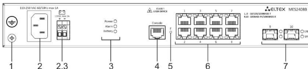
Figure 5 — MES2408B front panel
