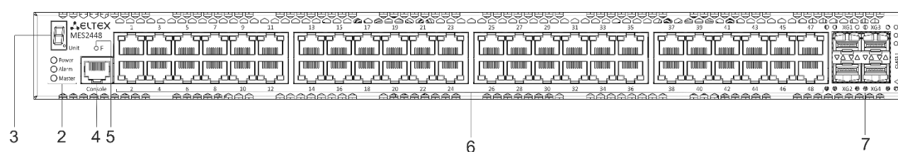
Figure 22 — MES2448 DC front panel
