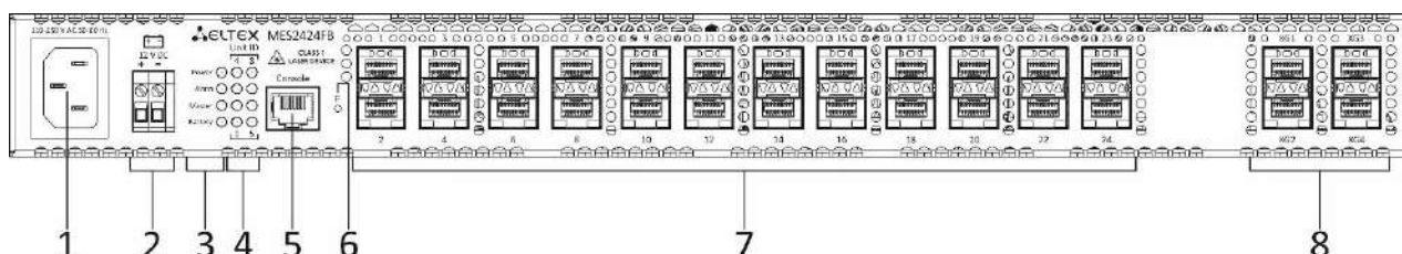
Figure 30 — MES2424FB front panel
