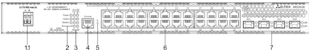
Figure 19 — MES2424 DC front panel
