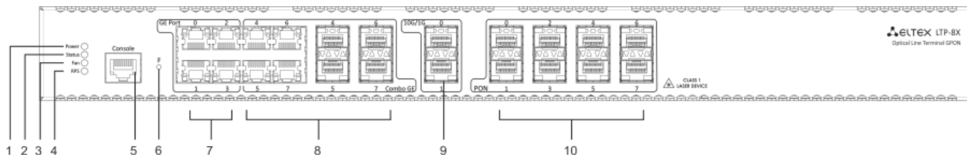
Figure 2 – Front panel of the LTP rev.C/rev.D
